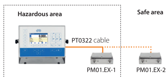
Block diagram of a system operating in hazardous area
